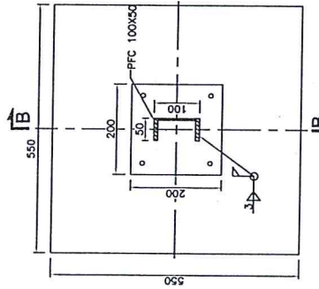
CONCRETE BLOCK DETAIL
